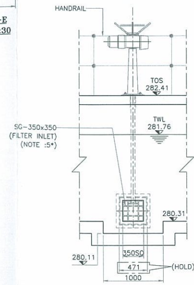
SECTION S7-S7 SCALE 1:30
