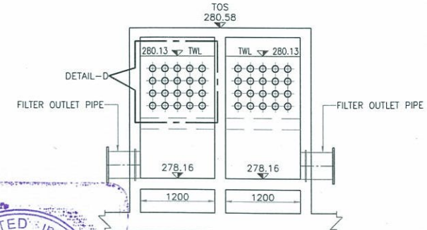
SECTION S6-S6 SCALE 1:40
