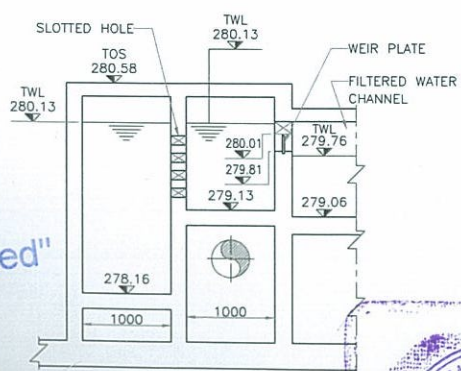
SECTION S5-S5 SCALE 1:40
