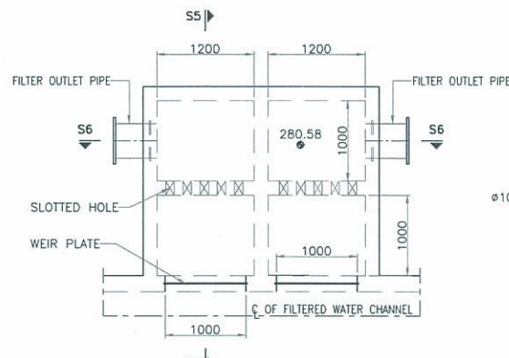
DETAIL-C SCALE 1:40
