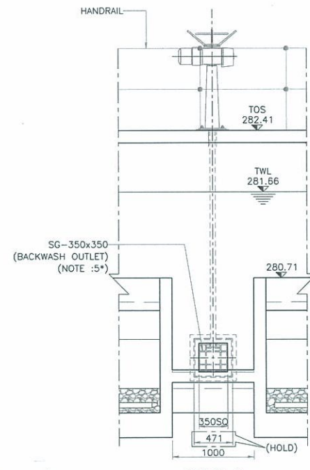
DETAIL-F SCALE 1:30
